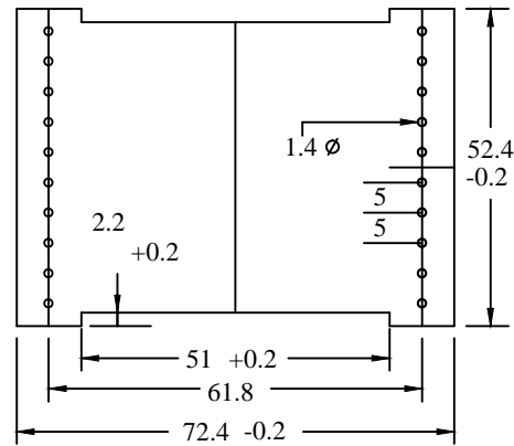
Horizontal PCB
